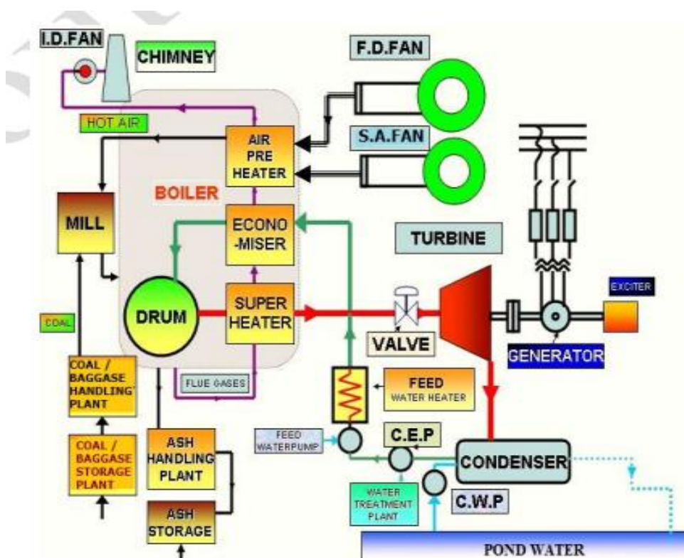
Figure 7: Typical Bagasse based power plant
